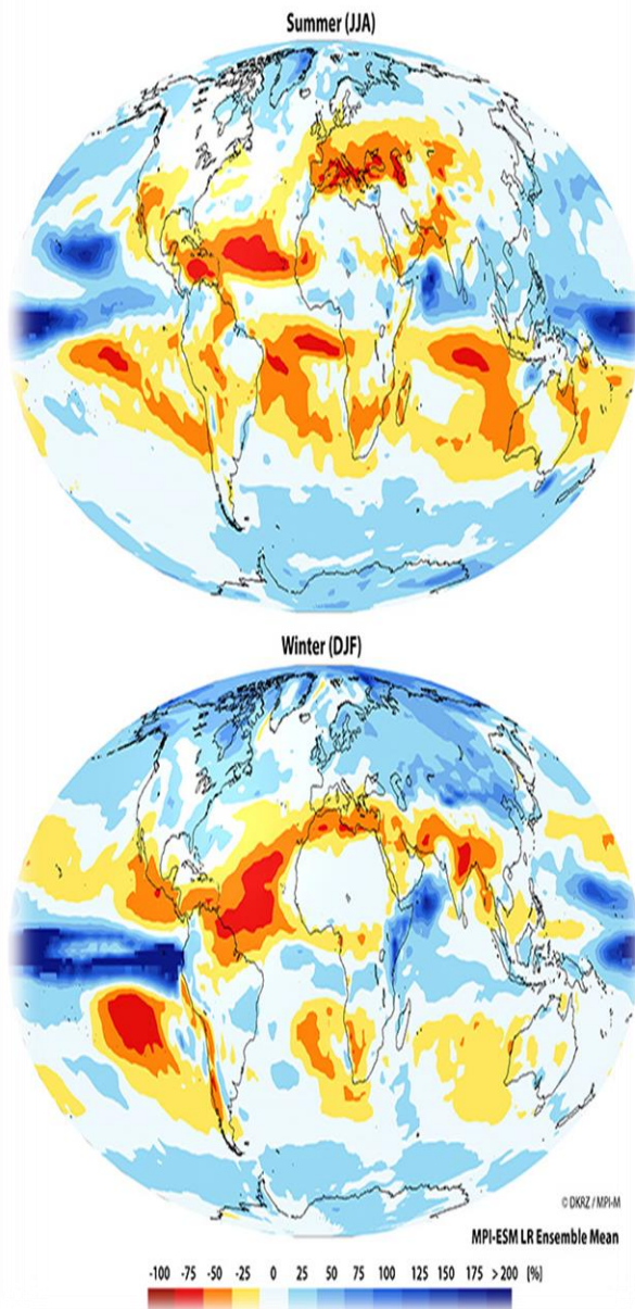
Figure 4 Simulated precipitation change in accordance with RCP 8.5 ( https://www.dkrz.de )
